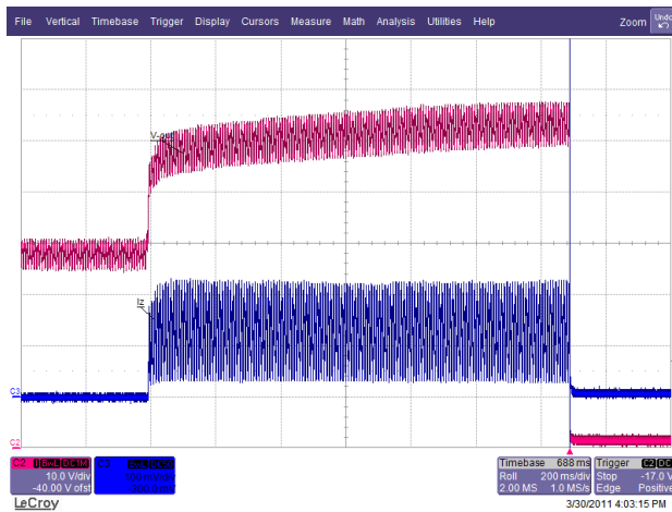
Figure 49 – 85 VAC / 63 Hz, Start-up No-load. Ch2: V_{OUT} , 10 V / div. Ch4: I_{OUT} , 100 mA / div., 200 ms / div.
