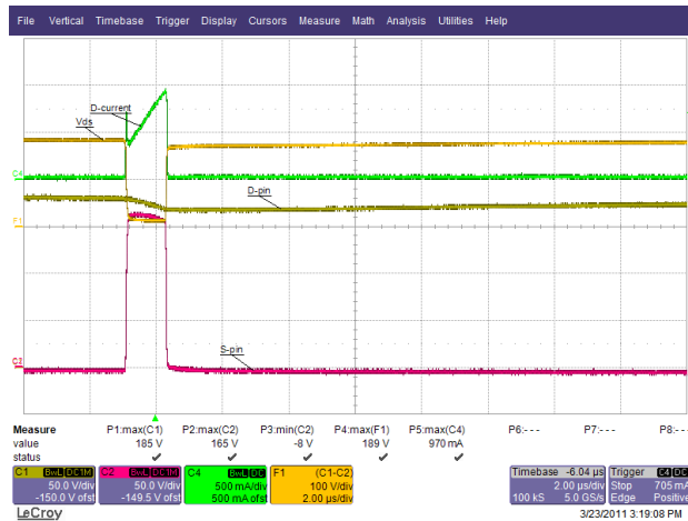
Figure 32 – 135 VAC / 63 Hz, 35 V LED String. Ch1: V_{DRAIN} , 50 V / div. Ch2: V_{SOURCE} , 50 V / div. Ch4: I_{DRAIN} , 0.5 A / div. F1: V_{D-S} , 100 V / div., 2 μs / div.
