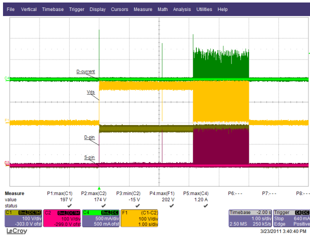
Figure 37 – 135 VAC / 63 Hz, Output Shorted. Ch1: V_{DRAIN} , 100 V / div. Ch2: V_{SOURCE} , 100 V / div. Ch4: I_{DRAIN} , 0.5 A / div. F1: V_{D-S} , 100 V / div., 1 s / div.
