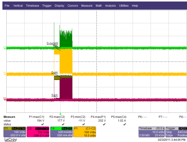
Figure 38 – 135 VAC / 63 Hz, Output Shorted. Ch1: V_{DRAIN} , 100 V / div. Ch2: V_{SOURCE} , 100 V / div. Ch4: I_{DRAIN} , 0.5 A / div. F1: V_{D-S} , 100 V / div., 10 s / div.
