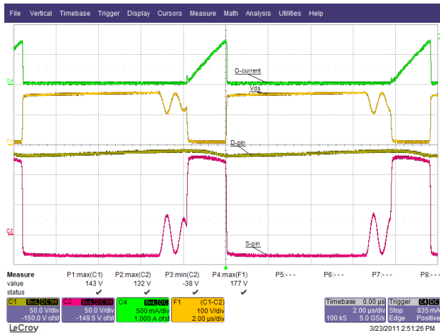
Figure 25 – 100 VAC / 50 Hz, 35 V LED String. Ch1: V DRAIN , 50 V / div. Ch2: V SOURCE , 50 V / div. Ch4: I DRAIN , 0.5 A / div. F1: V D-S , 100 V / div., 2 μs / div.
