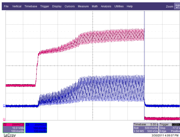
Figure 51 – 135 VAC / 63 Hz, Start-up No-load. Ch2: V_{OUT} , 10 V / div. Ch4: I_{OUT} , 100 mA / div., 500 ms / div.
