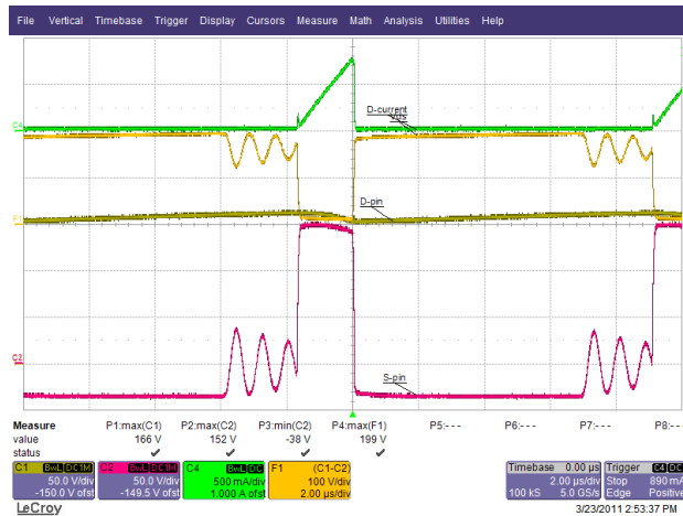
Figure 26 – 115 VAC / 60 Hz, 35 V LED String. Ch1: V DRAIN , 50 V / div. Ch2: V SOURCE , 50 V / div. Ch4: I DRAIN , 0.5 A / div. F1: V D-S , 100 V / div., 2 μs / div.
