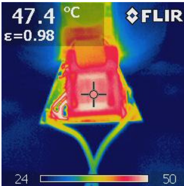
Figure 21 – L3 Temperature.
