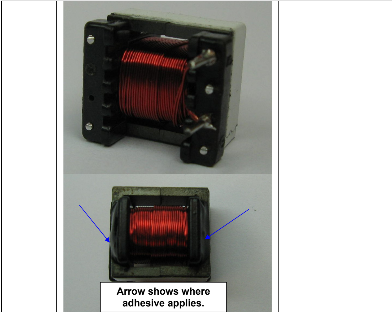
Figure 12 – Inductor Assembly.
