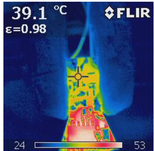
Figure 22 – BR1 Case Temperature.
