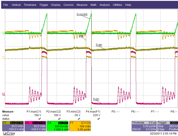
Figure 27 – 135 VAC / 63 Hz, 35 V LED String. Ch1: V_{DRAIN} , 50 V / div. Ch2: V_{SOURCE} , 50 V / div. Ch4: I_{DRAIN} , 0.5 A / div. F1: V_{D-S} , 100 V / div., 5 \mu s / div.
