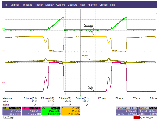
Figure 23 – 85 VAC / 47 Hz, 35 V LED String. Ch1: V DRAIN , 50 V / div. Ch2: V SOURCE , 50 V / div. Ch4: I DRAIN , 0.5 A / div. F1: V D-S , 100 V / div., 2 μs / div.
