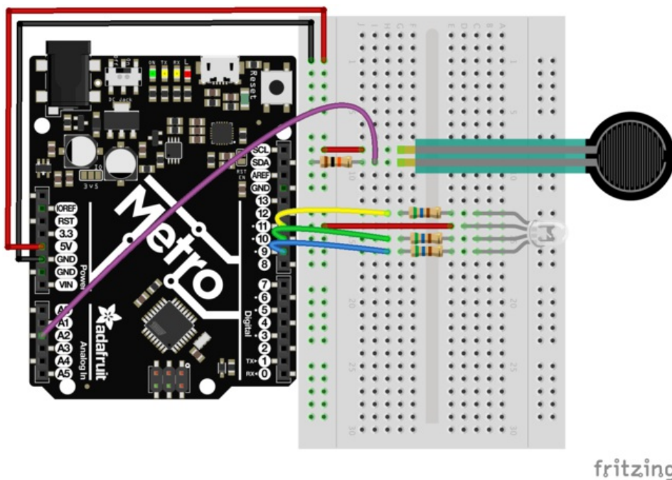
Diagram: RGB + Force Resistor
