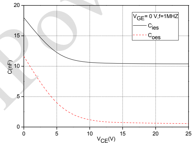
Fig.4 Capacitance Characteristics
