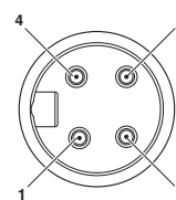
Pin assignment, plug, 7/8"-16UNF, 4-pos., view of male side
